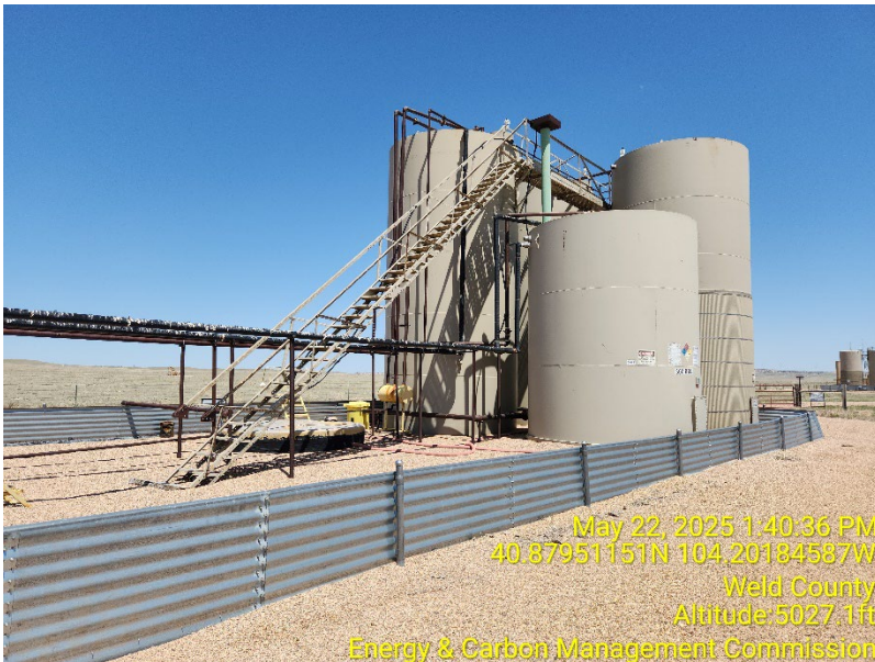
Photo 1 – Tank Battery
