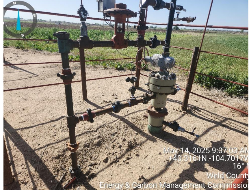
Photo 4 well head and equipment
