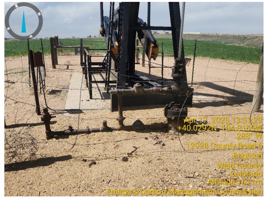
Photo 2 Wellhead.
