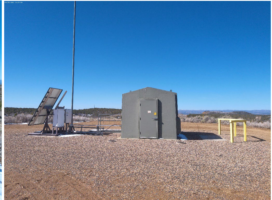
Injection Wellhead inside housing
