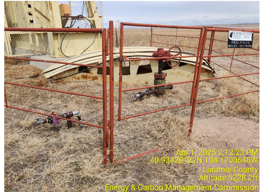
Photo 2 – Wellhead
