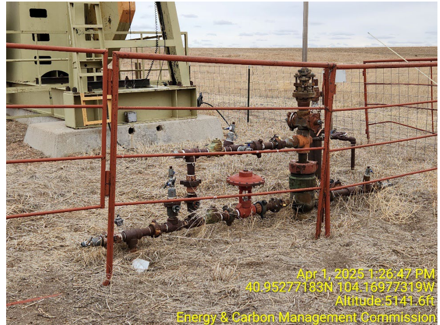
Photo 6 – Wellhead
