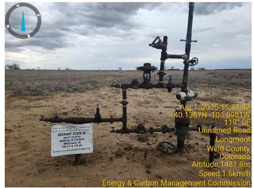
Photo 2 Wellhead & sign.
