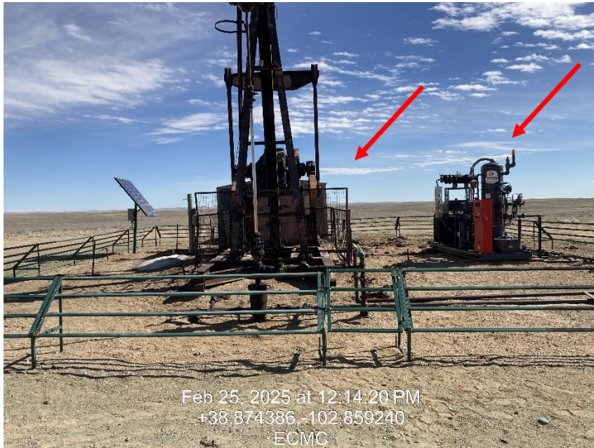
Photo 7 –Wellhead and equipment
