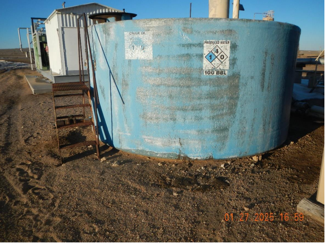
Double labeled tank. Stained ground. No berming around tank.
