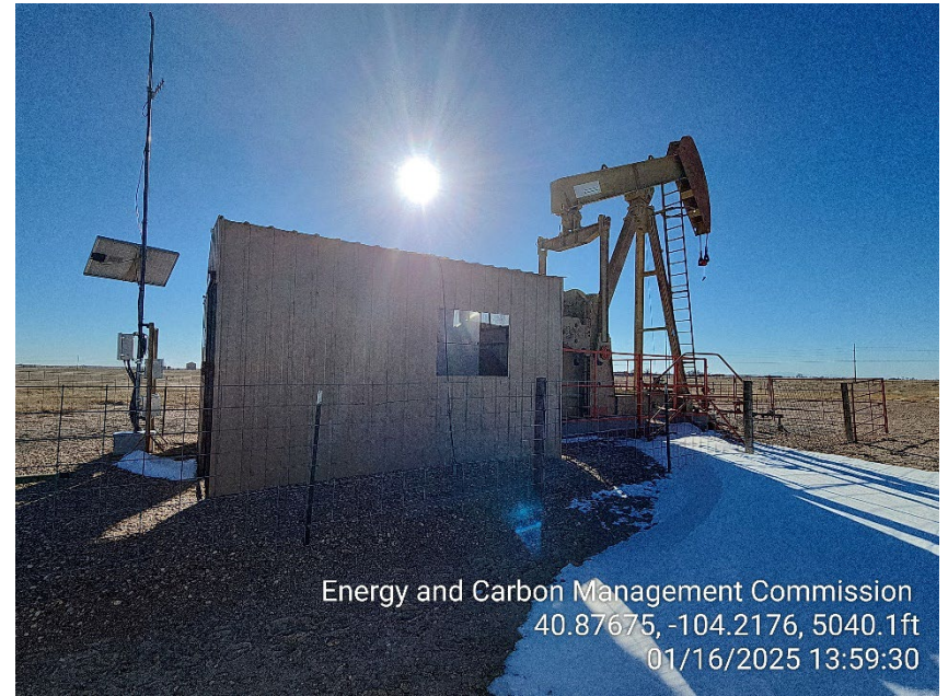
Photo 2 – Pumping Unit
