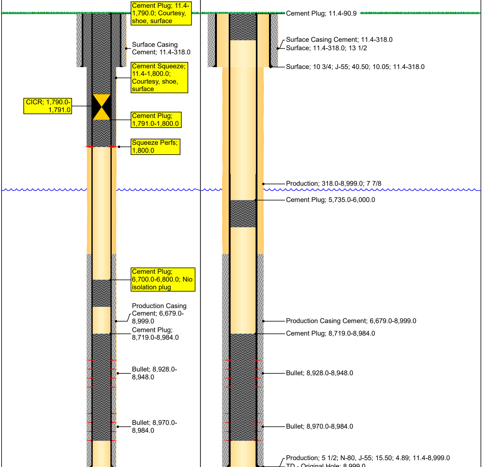
Vertical schematic (proposed)
