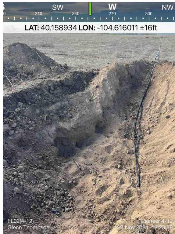
FL02(4-12)@5'
