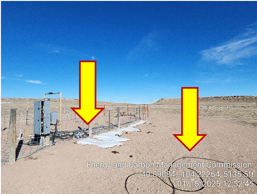
Photo 1 – Unused Automation Equipment
