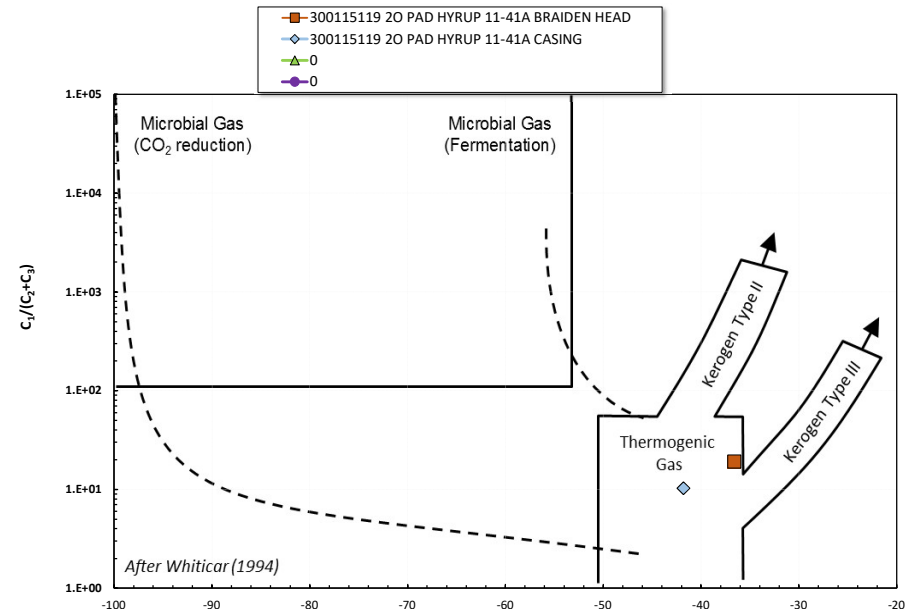
Methane \delta^{13}\text{C} vs C1/(C2+C3) Genetic Classification Plot
