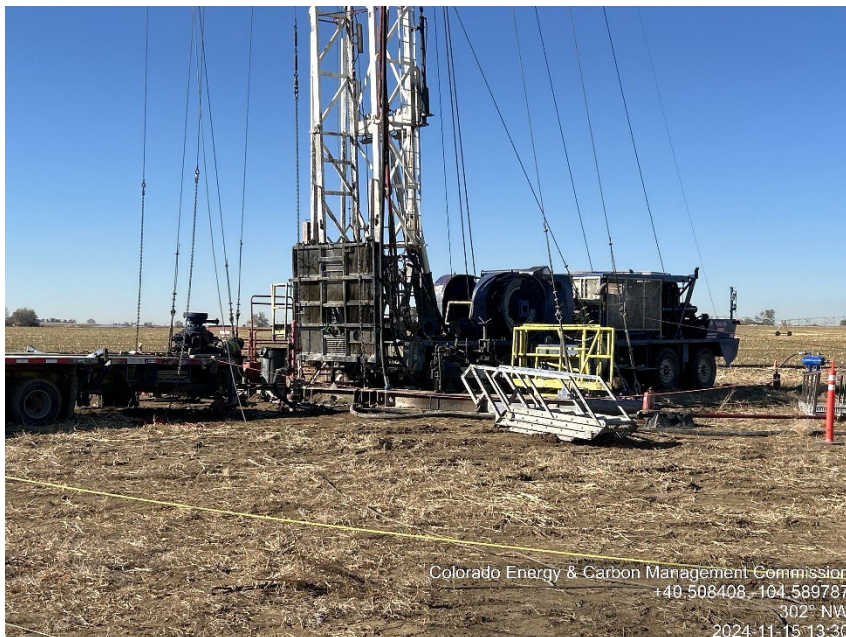
Photo #1 Kreps Trust 34-6 (123-21723) Wellsite Workover | WK Plugging Ops: Kill well, flare gas
