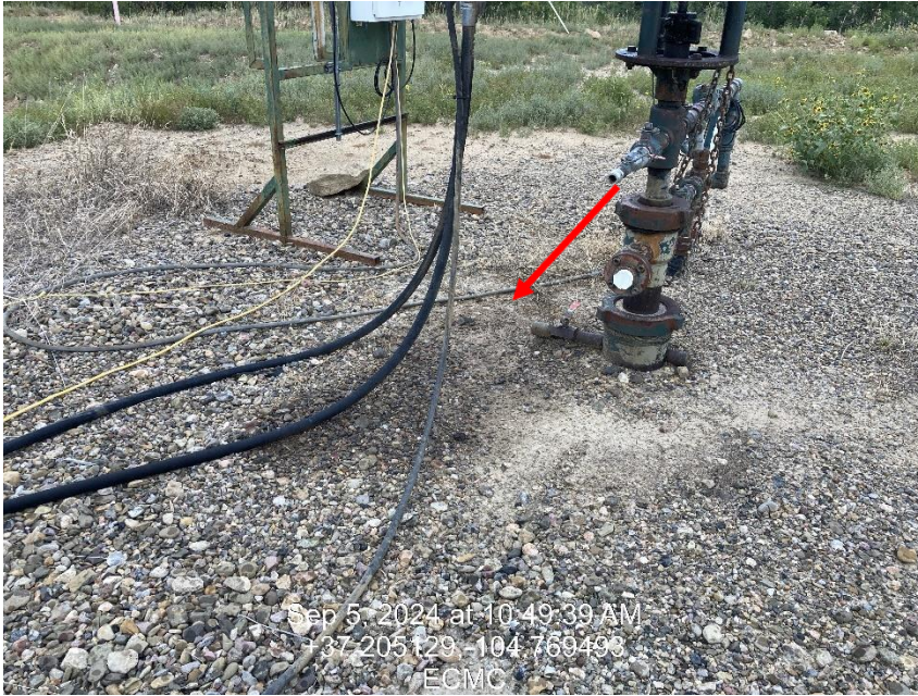
Photo 3 – Oil stained soils at wellhead
