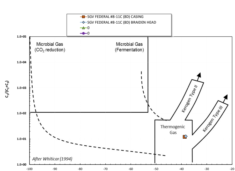
Methane \delta^{13}C vs C1/(C2+C3) Genetic Classification Plot
