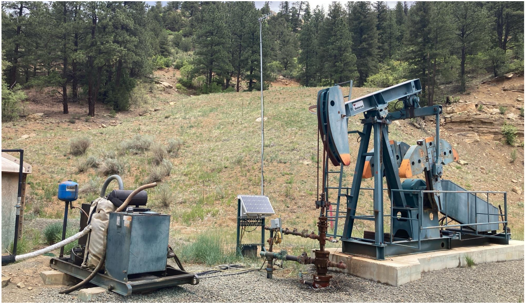
PHOTO 3: WELLHEAD AND EQUIPMENT/ PACKING ON V WELL IS LEAKING
