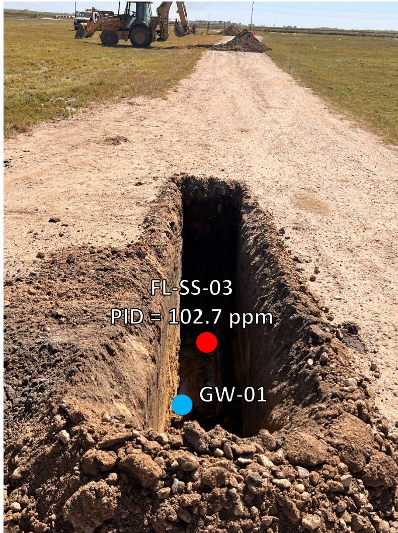
Looking south at bellhole/cut point for removal
