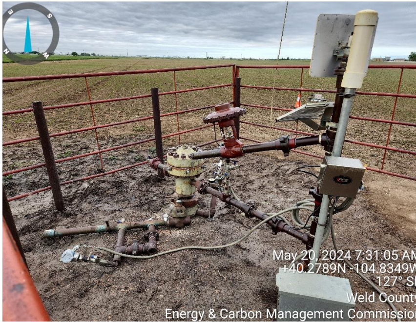
Photo 7, 5-20-24 well head and equipment
