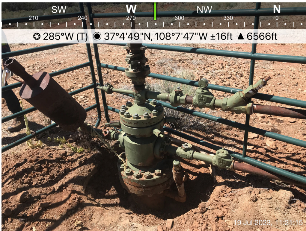
Photo 2: Turner (OWP) #4 wellhead, 7/19/2023.
