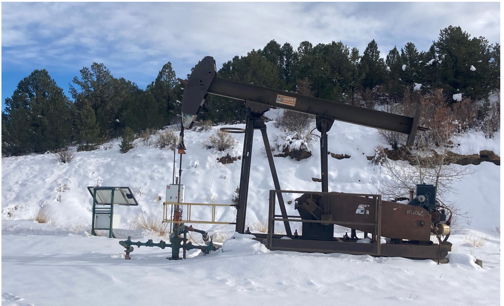
PHOTO 3: WELLHEAD AND EQUIPMENT
