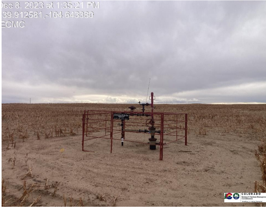
Pic 1 Wellhead
