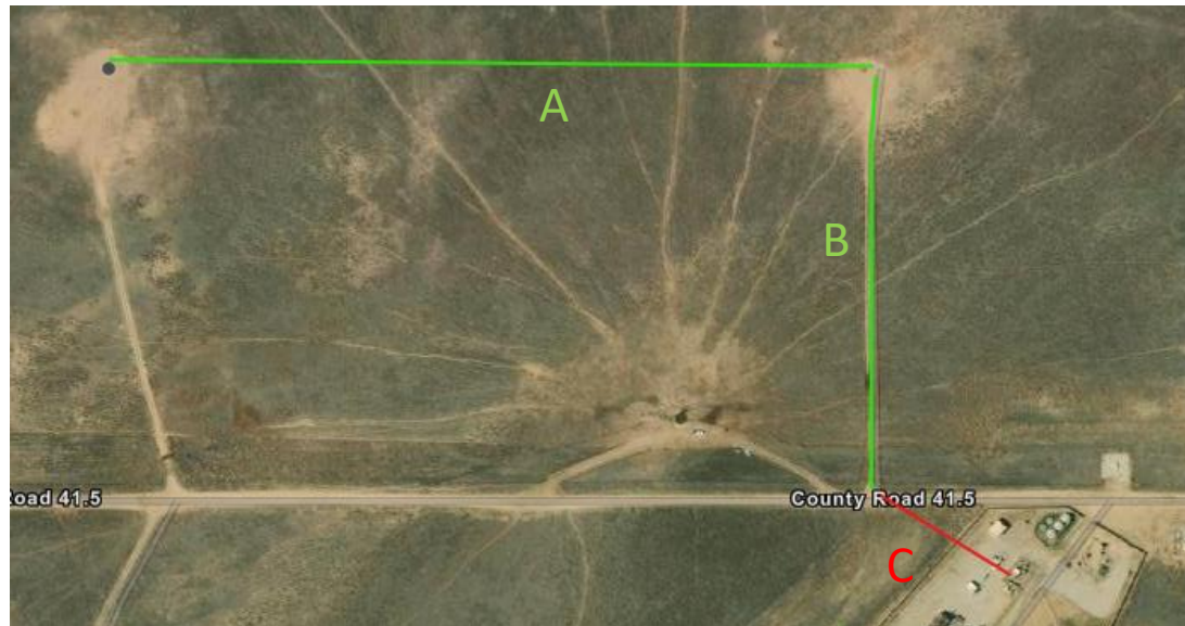
12313662_FL / 1231365912316572_FL Segment Map: Planned Flowline Abandonments
