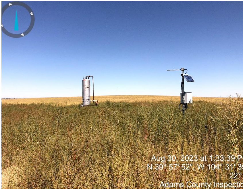
Photo #3 Meter & Separator.
