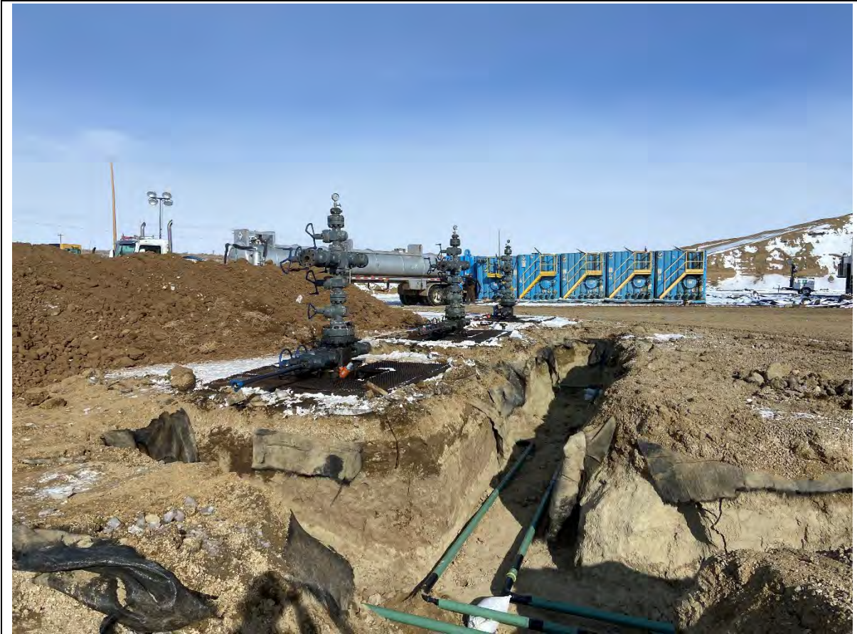
PHOTO NO 3: VIEW OF NEWLY INSTALLED WELLHEADS. LOOKING NORTH.
