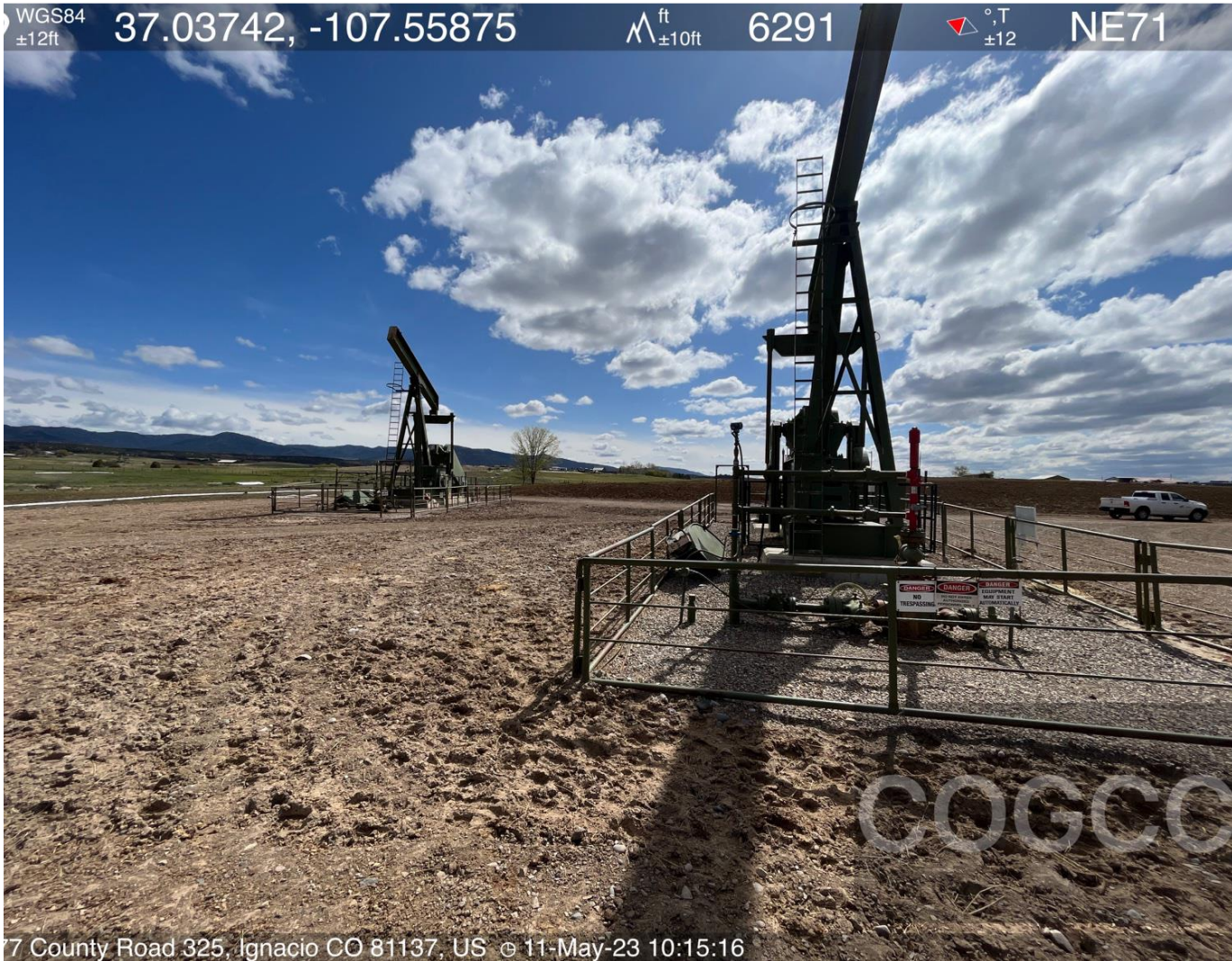
Photo #2. View of wellheads and pumpjacks..
