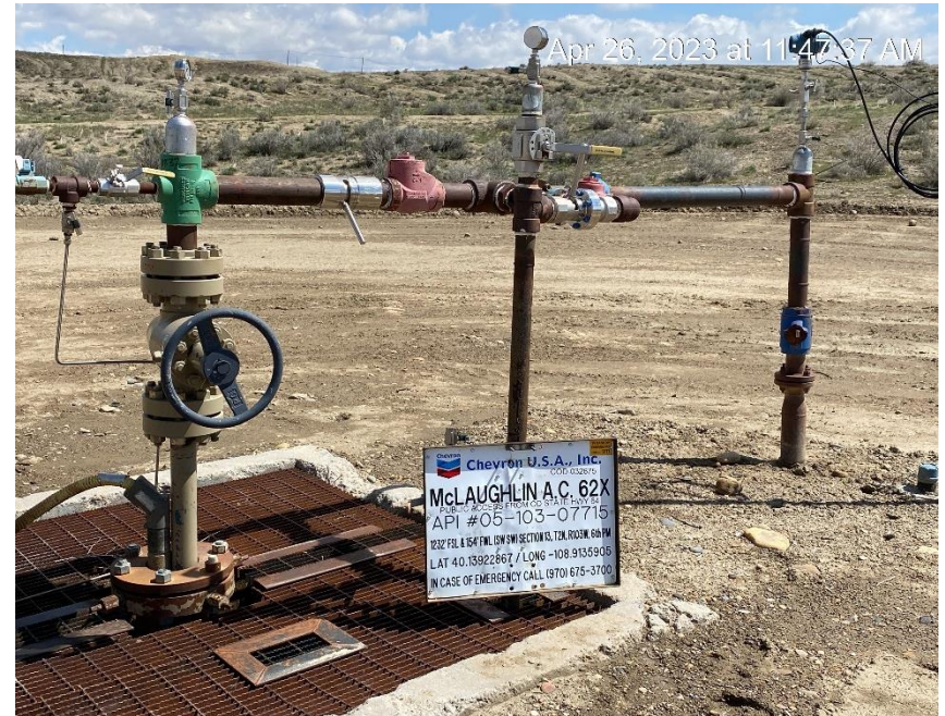
Wellhead and location sign
