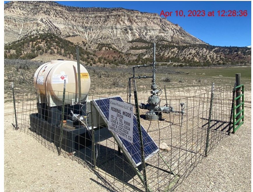
Wellhead – Photo #02009
