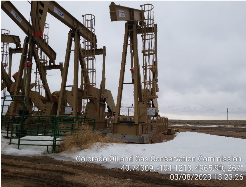
Photo 3 – Unused Pumping Unit at 3-17 Wellsite
