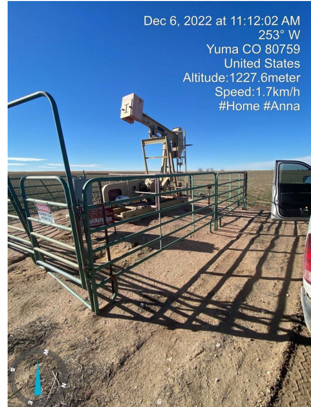
2. Wellhead Equipment
