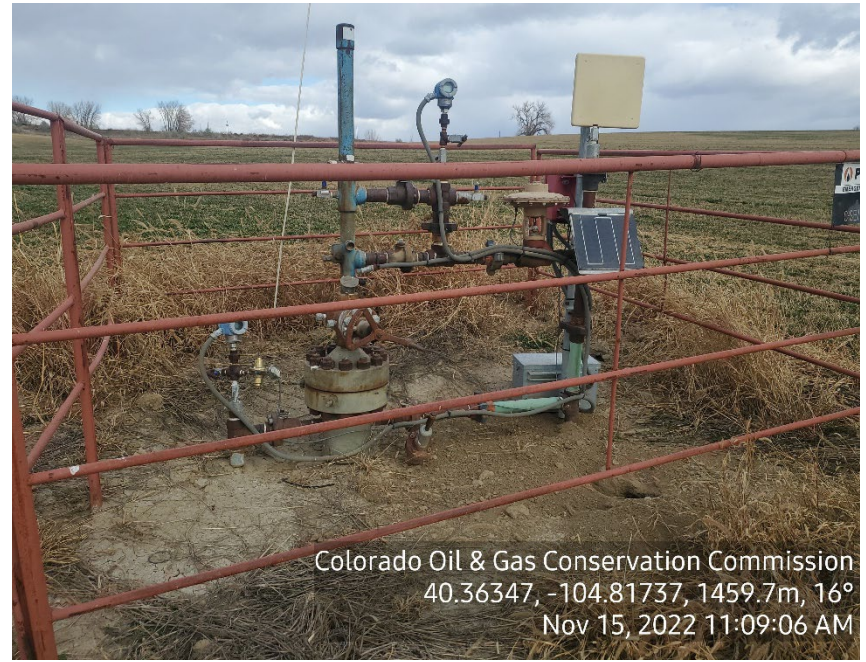
Photo 2: Wellhead
