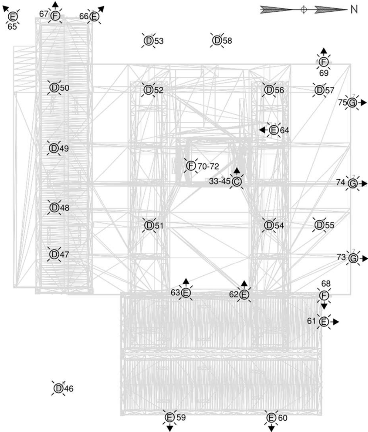
LUMINAIRE LAYOUT BAYSWATER GARNET 21-K – DRILL AREA – DETAIL B PRE-PRODUCTION – CONSTRUCTION DRILLING OPERATIONS
