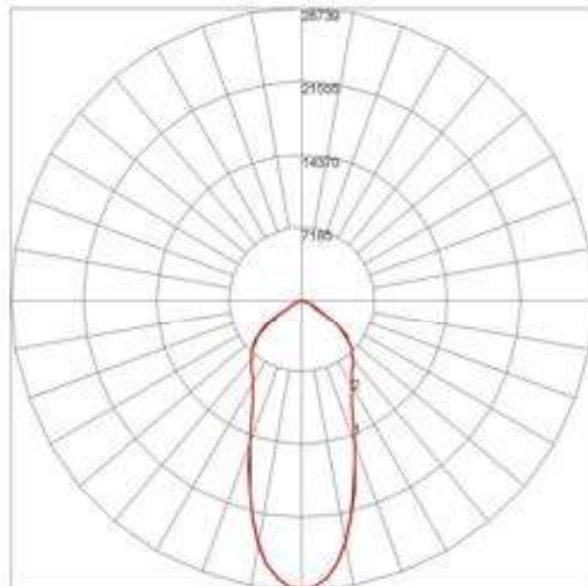
Maximum Candela = 28730.4 - Located At Horizontal Angle = 0, Vertical Angle = 0 # 1 - Vertical Plane Through Horizontal Angles (0 - 180) # 2 - Vertical Plane Through Horizontal Angles (90 - 270)
