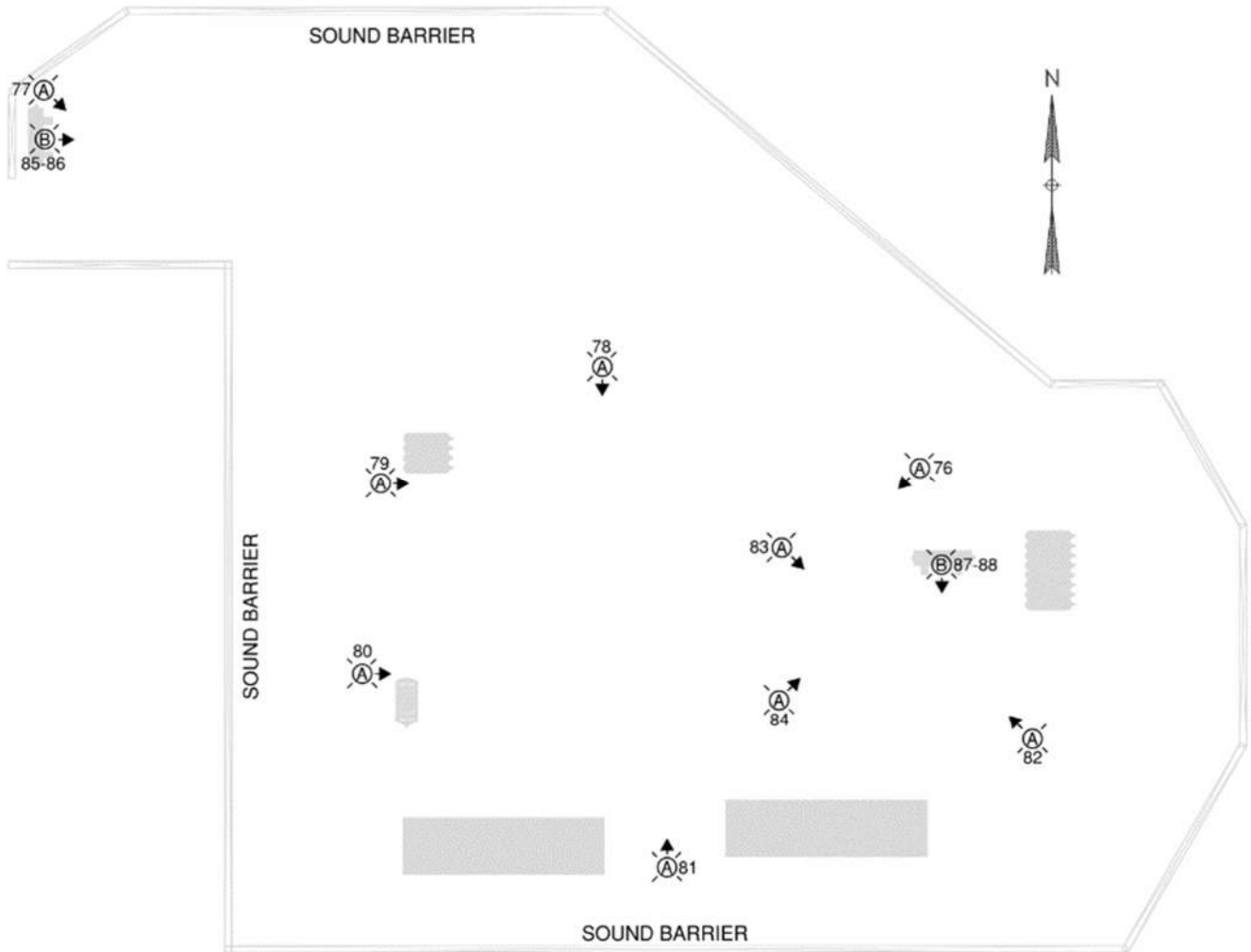
LUMINAIRE LAYOUT BAYSWATER GARNET 21-K – COMPLETIONS PRE-PRODUCTION – CONSTRUCTION
