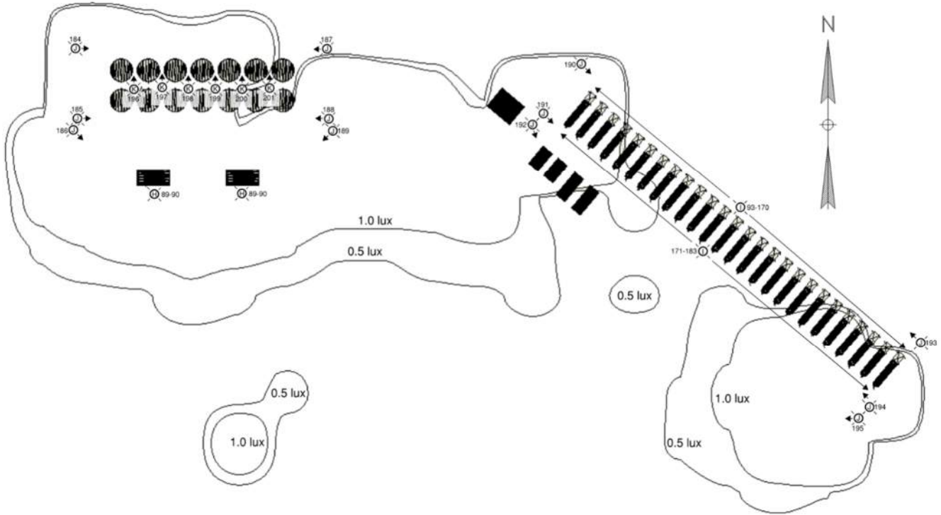
LUMINAIRE LAYOUT & PHOTOMETRIC BAYSWATER GARNET 21-K – PRODUCTION AREA PRODUCTION OPERATIONS
