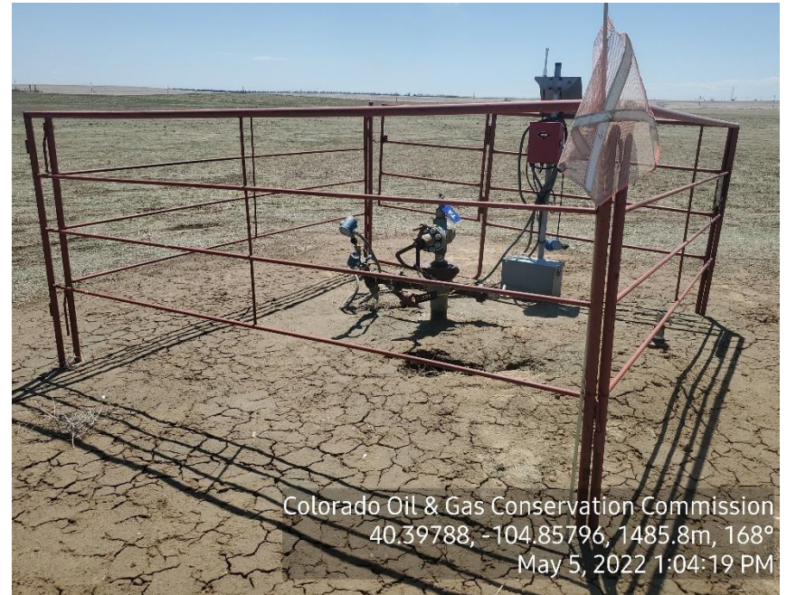
Photo 2: TA Wellhead
