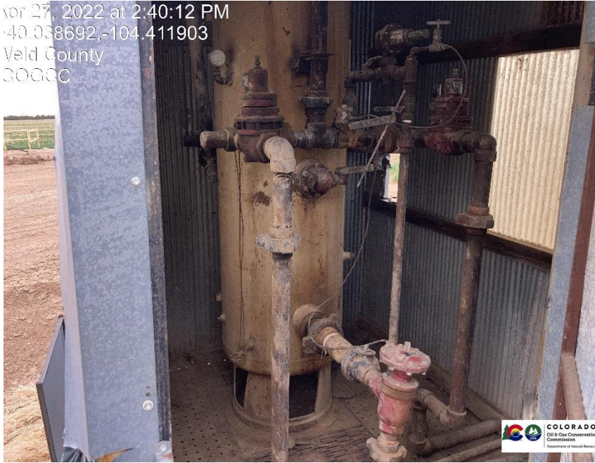
Pic 3 separator
