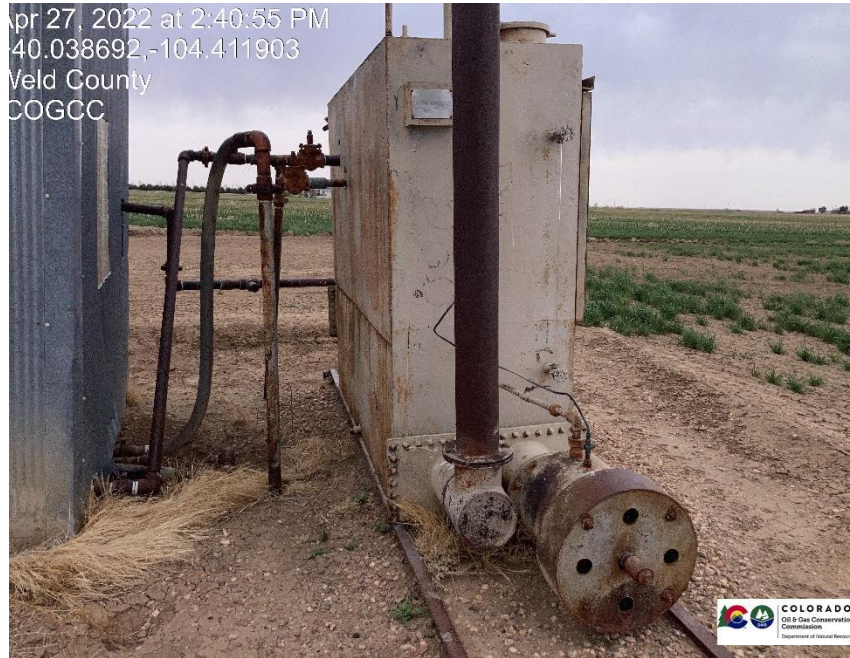
Pic 5 separator
