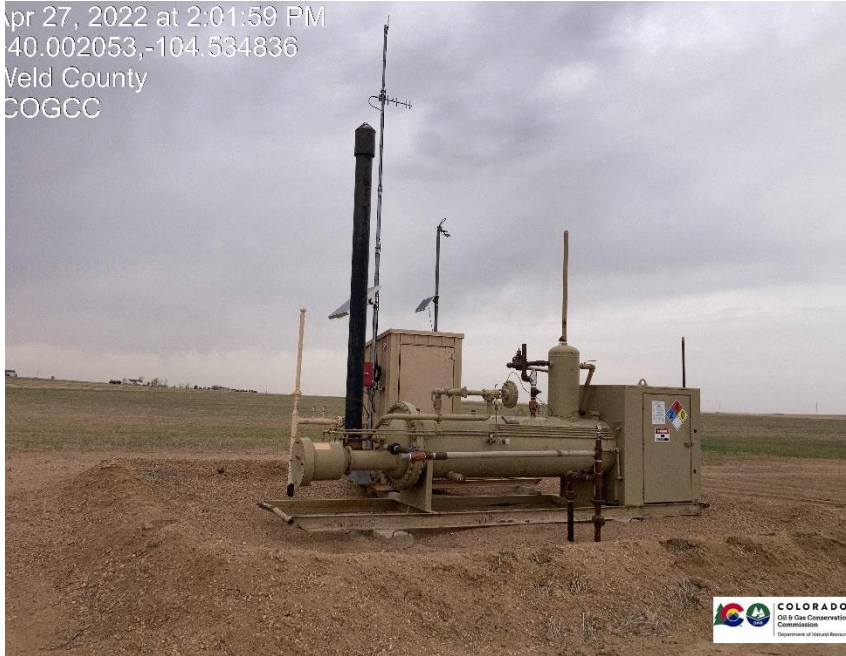
Pic 3 gas meter run, separator
