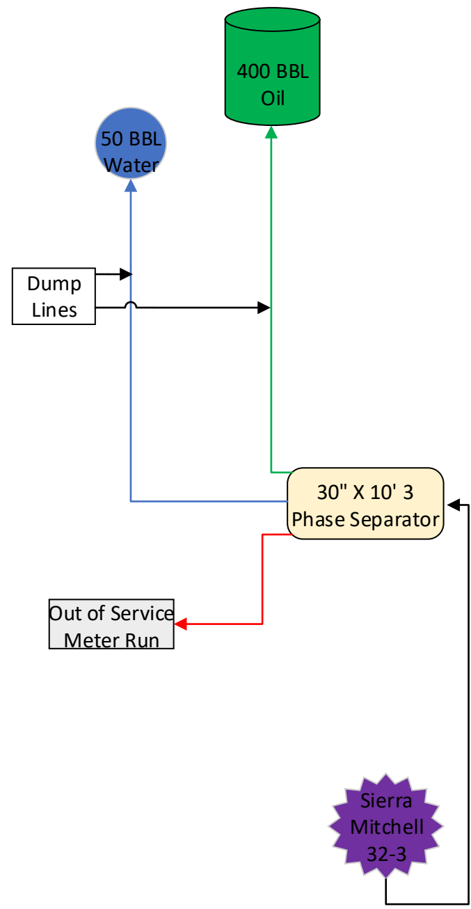
Sierra Mitchell #32-3 Battery Process Flow Diagram NESW Section 32 - 4S - 63W Arapahoe Co., CO
