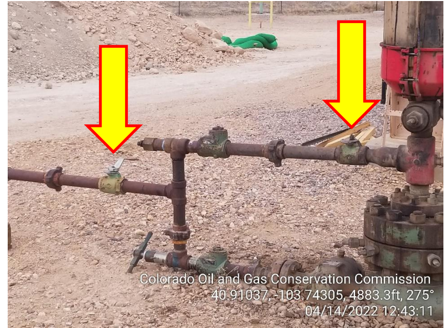
Photo 2 – Wellhead – Tubing Valves appear to be Closed Position
