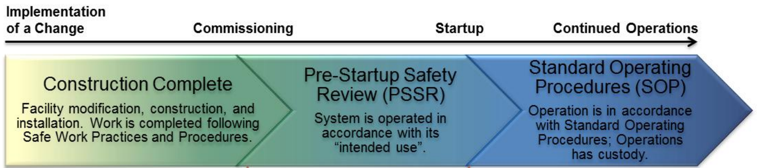
Figure 3: PSSR Timing
