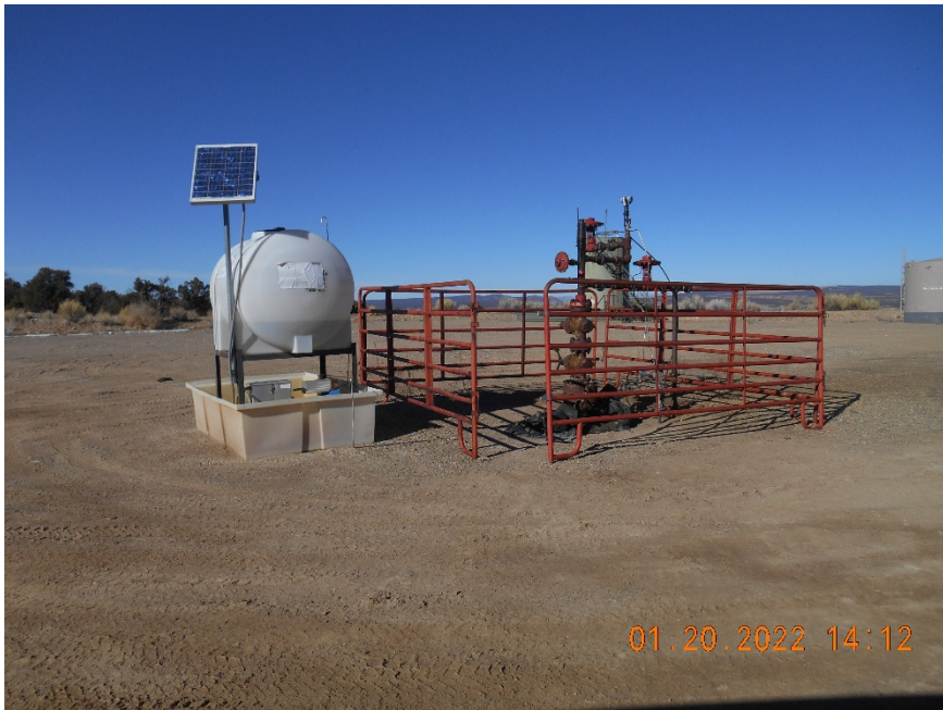
Wellhead with fence. Secondary containment of chemicals
