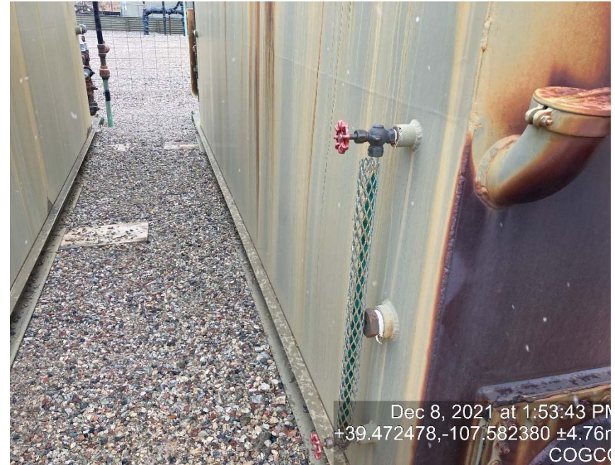
Unmarked vessels show level of fluid in sight glass
