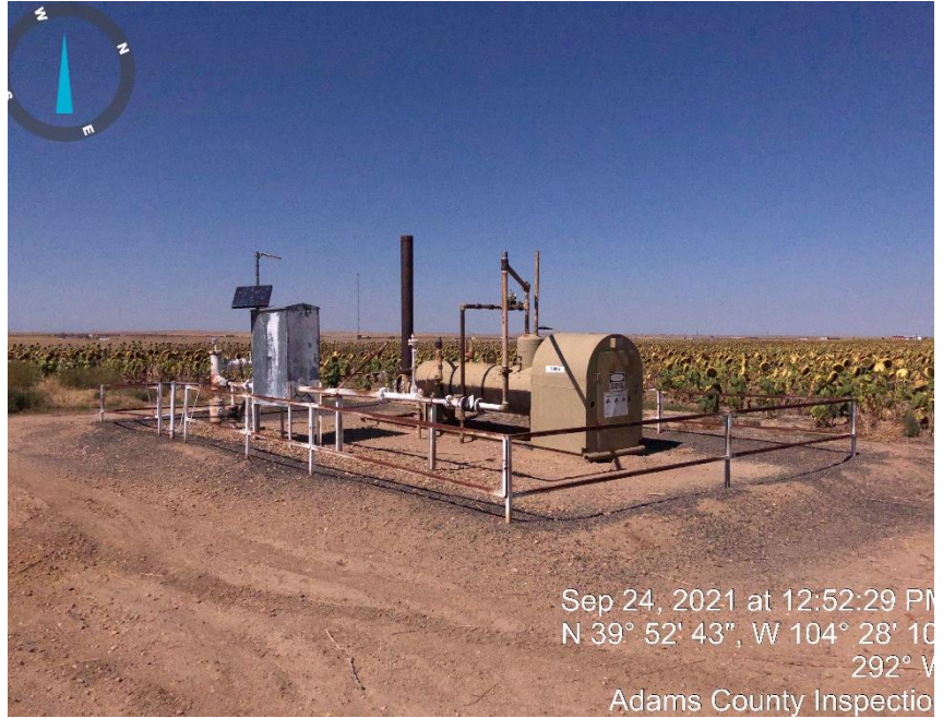
Photo #2 Separator and meter.
