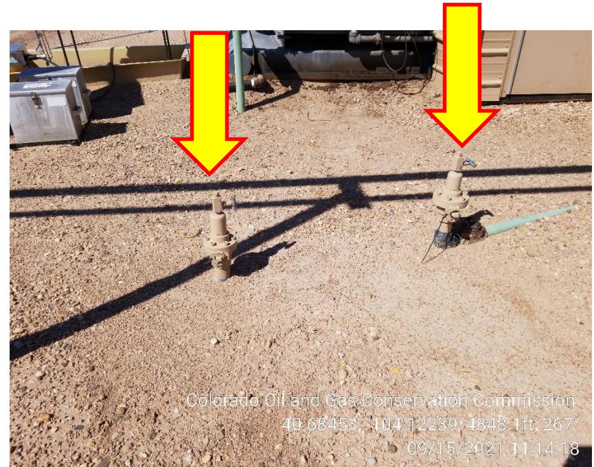
Photo 6 – Unmarked Risers at Compressor
