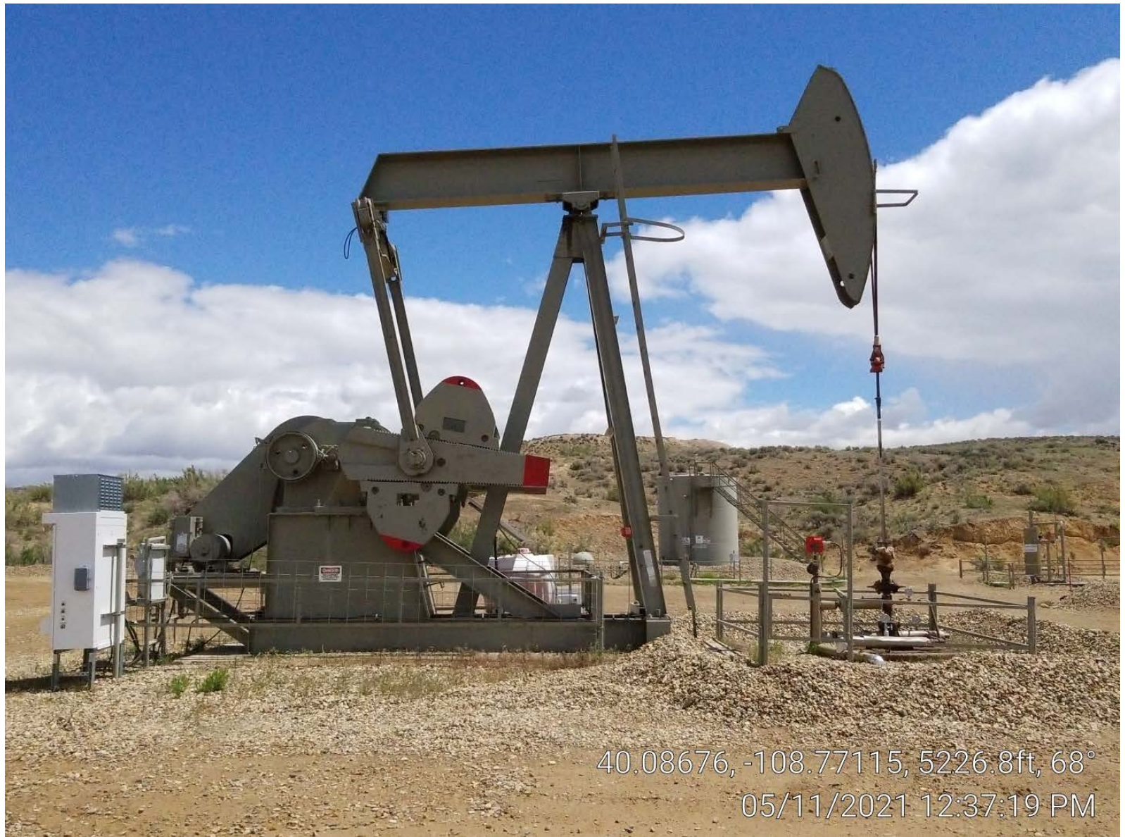
Photo 2. Pump jack.
