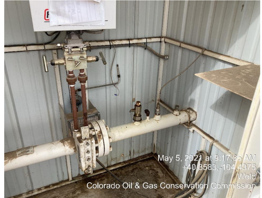
Photo #4 Removed Mechanical condition.
