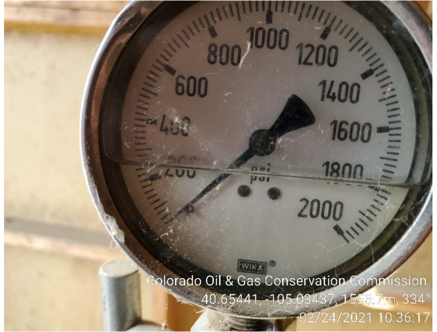
Casing pressure
