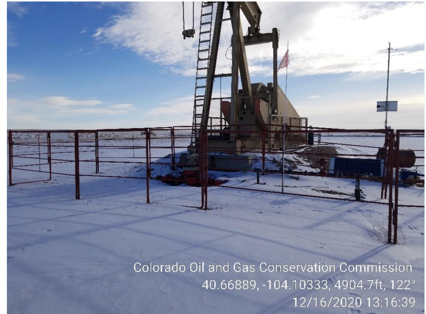
Photo 2 – Pumping Unit
