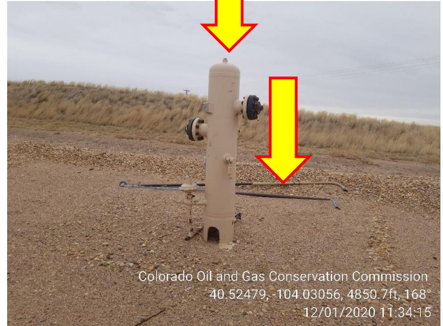
Photo 8 – Unused Supply Pot and 1” pipe
