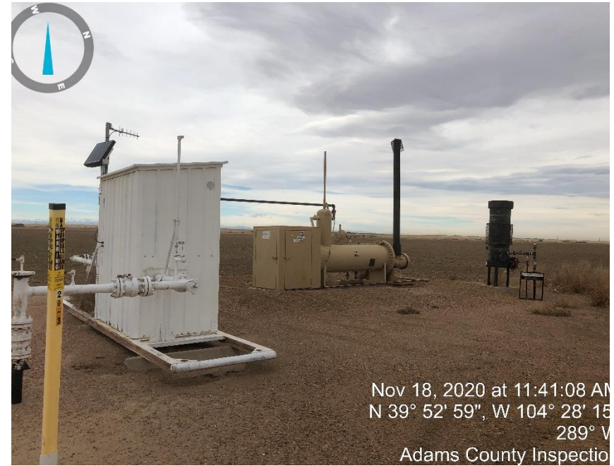
Photo #2 Meter, Separator, ECD.
