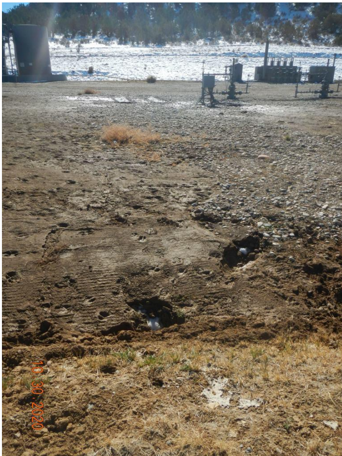
Photo#4: Stormwater tunneling through sink holes off ditches and pooling areas.
